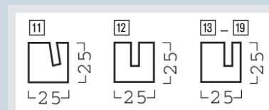
Abmessungen in mm
